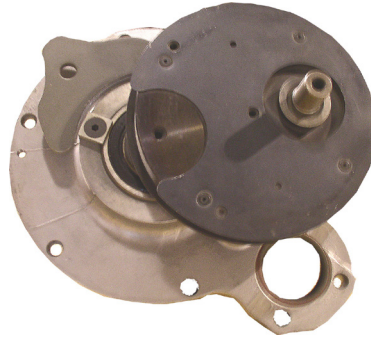
Deck Lift Crank Assembly 2-1 Assembly
