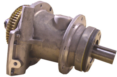
Rake Crank Housing Assembly 4-1 Assembly
