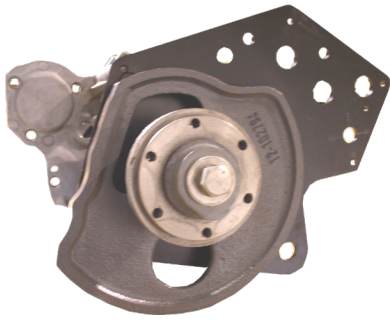
Gearbox Cover Assembly 1-1 Assembly
